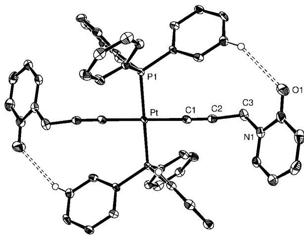
Figure 3. Molecular structure of trans -[Pt(C≡CCH 2 R 1 ) 2 (PPh 3 ) 2 ] (1). Thermal ellipsoids show 50% probability levels. Hydrogen atoms (except those involved in H-bonding interactions) omitted for clarity.
